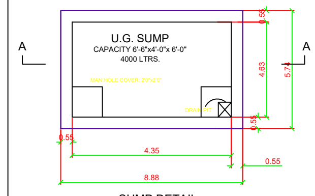
SUMP DETAIL
