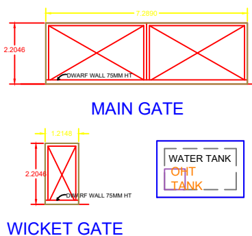
WICKET GATE
