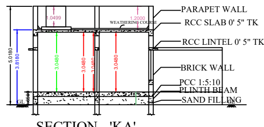
SECTION - 'KA'
