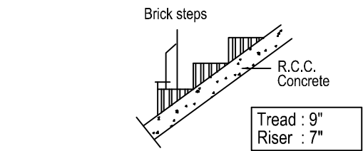
STAIRCASE DETAILS
