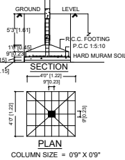
COLUMN SIZE = 0'9" X 0'9"
