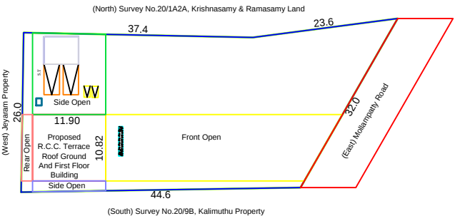
SITE PLAN (Scale 1: 400)
