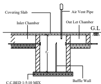
SECTION ON S.Tank
