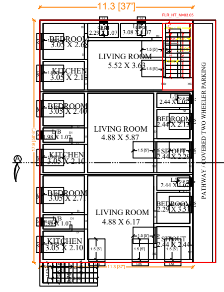
EXIS. GROUND FLOOR PLAN (1ST, 2ND & 3RD DWELLING UNIT)
