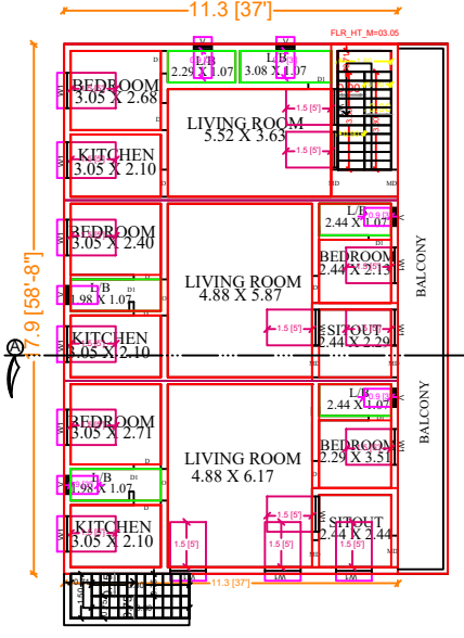
SECOND FLOOR PLAN (7TH, 8TH DWELLING UNIT & 9TH UNIT)
