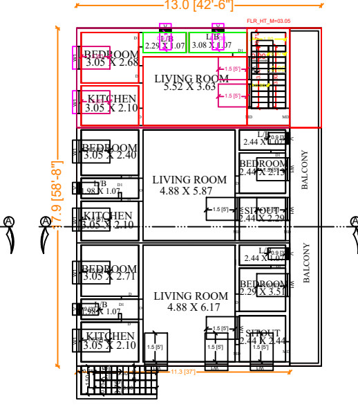
EXIS. FIRST FLOOR PLAN & PROPO. FIRST FLOOR PLAN (3RD HOUSE) (4TH, 5TH & 6TH DWELLING UNIT)
