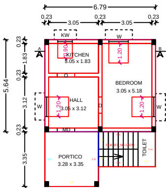
PROPOSED GROUND FLOOR PLAN NORTH FACING
