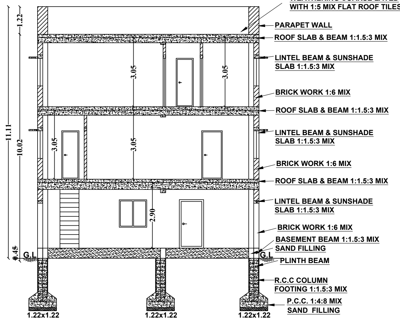
SECTION "AB".
