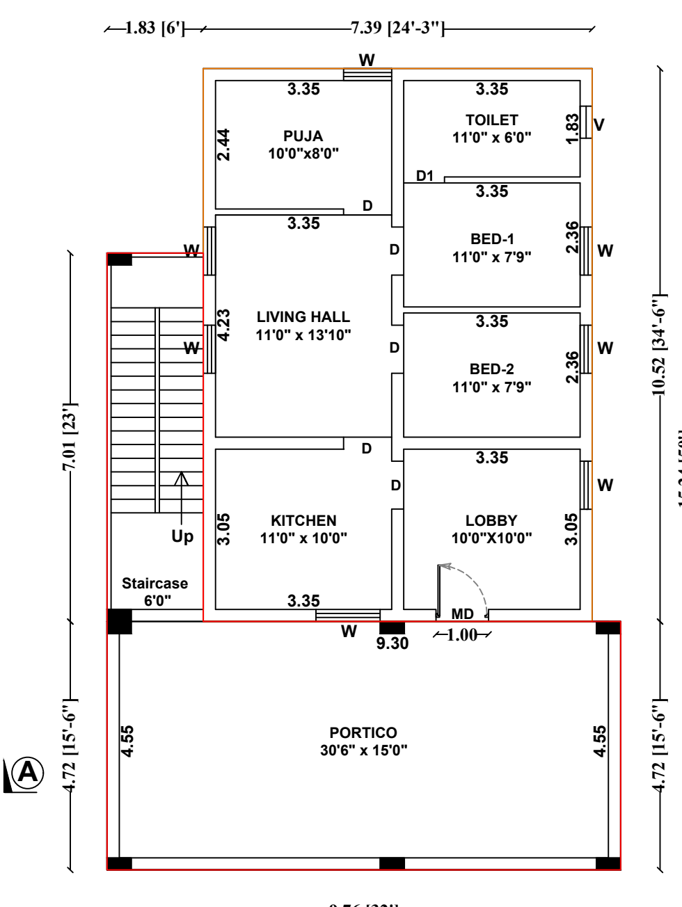
EXISTING GROUND + PROPOSED STILT FLOOR PLAN.
