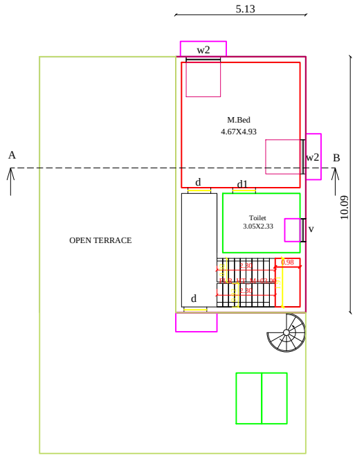
FIRST AND TERRACE FLOOR PLAN
