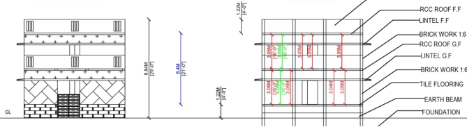
FRONT ELEVATION
