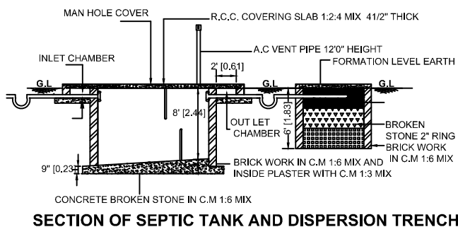
SECTION OF SEPTIC TANK AND DISPERSION TRENCH
