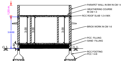
SECTION-"SR"
