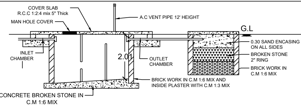
SECTION OF SEPTIC TANK AND SOAK PIT
