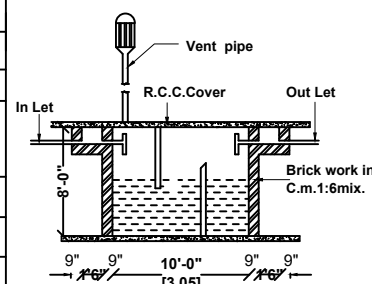
SEPTIC TANK DETAILS (NOT TO SCALE)
