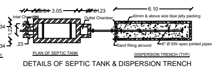
DETAILS OF SEPTIC TANK & DISPERSION TRENCH
