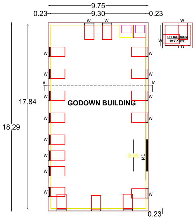
PROPOSED GROUND FLOOR PLAN GODOWN BUILDING FACING NORTH
