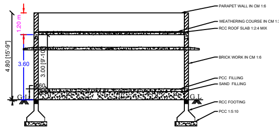
SECTION ON - "SR"
