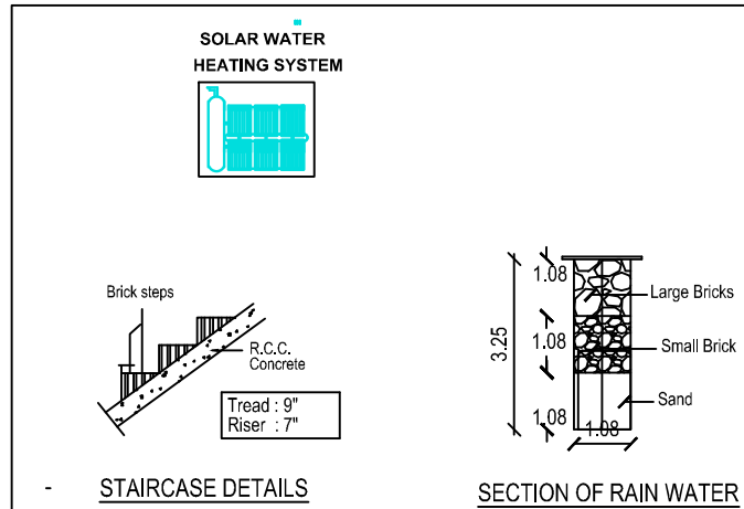
STAIRCASE DETAILS
