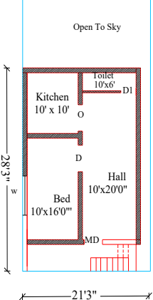
Proposed Second Floor
