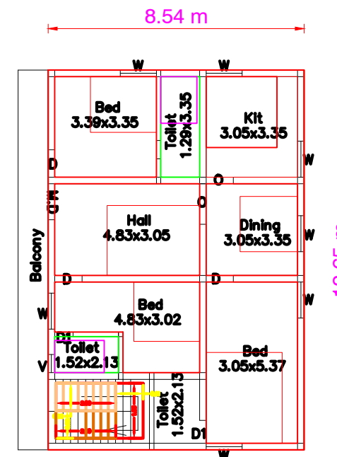
FIRST FLOOR(Pro.)
