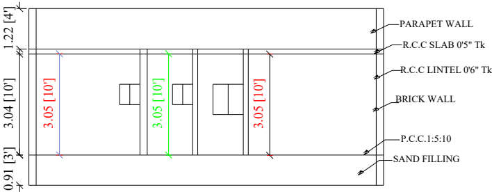
SECTION ON"AB"
