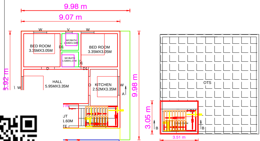
FIRST FLOOR(Pro.)
