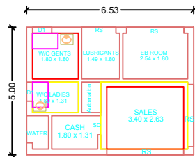
PRO.GROUND FLOOR PLAN
