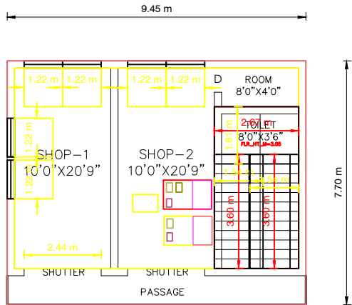
FIRST FLOOR PLAN [SOUTH FACING]
