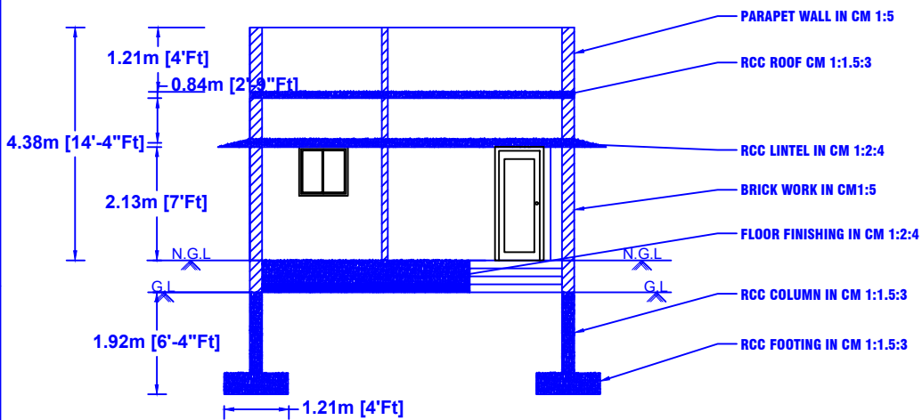
SECTION ON-AA
