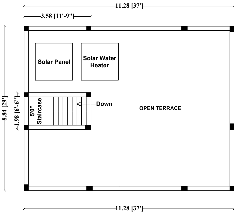
.TERRACE FLOOR.
