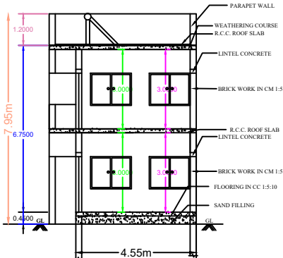
SECTION AB
