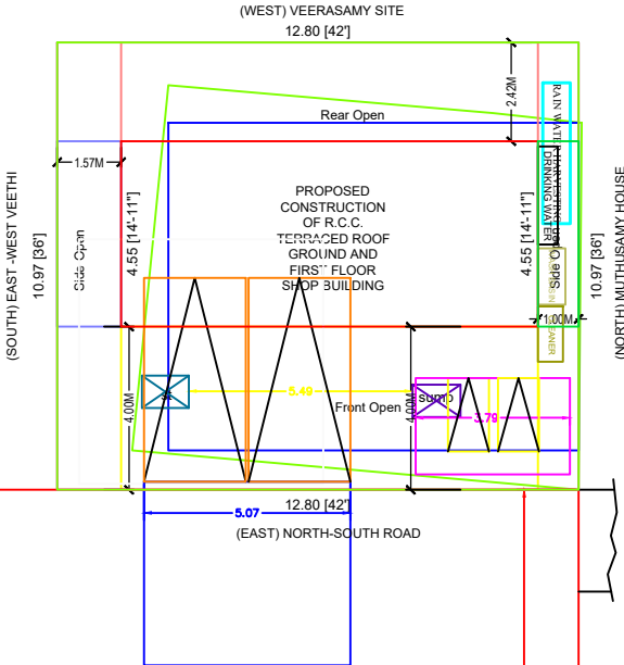
SITE PLAN
