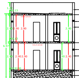
SECTION ON K-S
