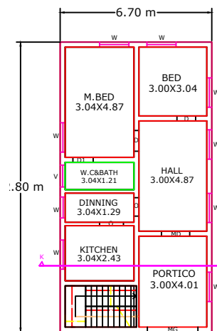
POSED GROUND FLOOR PLAN
