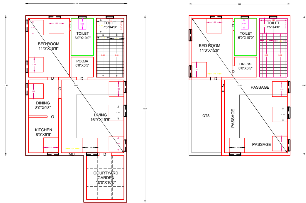
GROUND FLOOR PLAN [EAST FACING]
