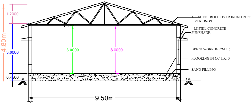
SECTION AB
