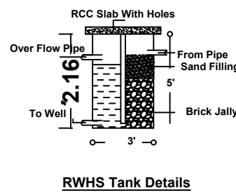
Solar Water Tank Details
