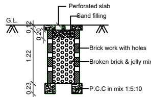
PERCOLATION PIT FOR 30 Sq. m. (Scale:- 1:50)
