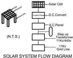
SOLAR SYSTEM FLOW DIAGRAM
