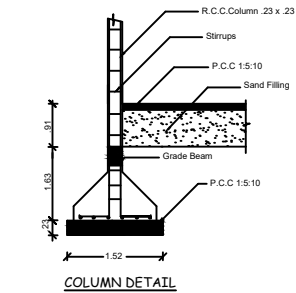
COLUMN DETAIL
