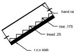
STAIR
