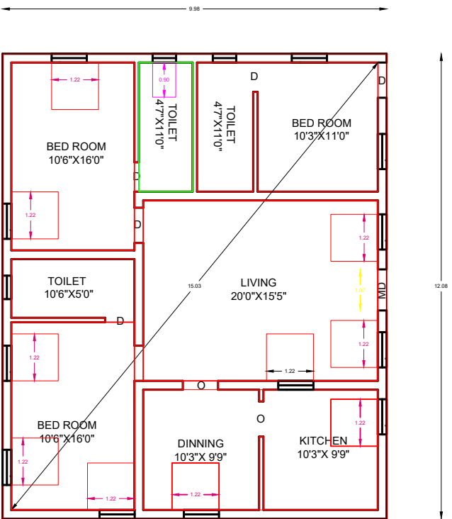
GROUND FLOOR PLAN [SOUTH FACING]
