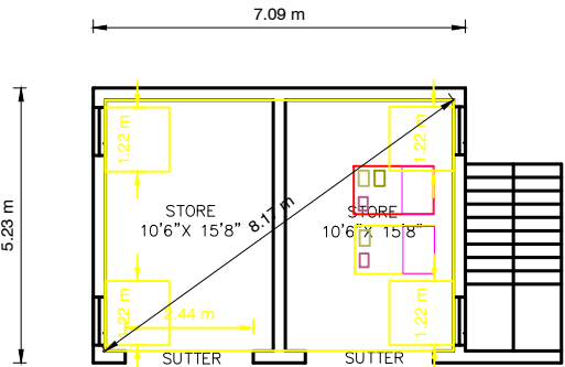
GROUND FLOOR PLAN [SOUTH FACING]
