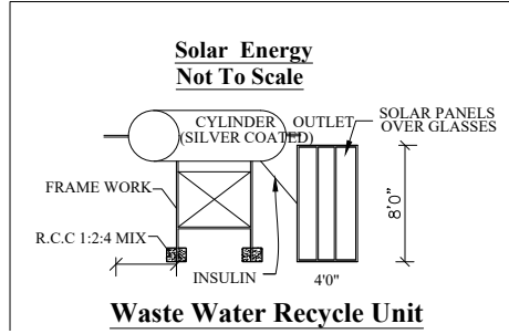
Waste Water Recycle Unit Not To Scale
