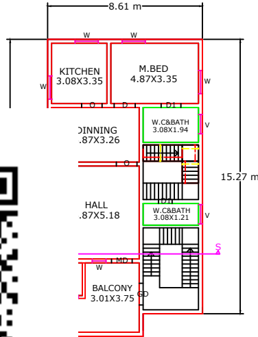
ED FIRST FLOOR PLAN
