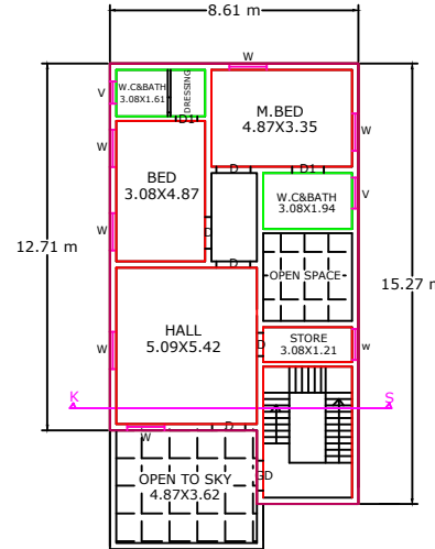
PROPOSED SECOND FLOOR PLAN
