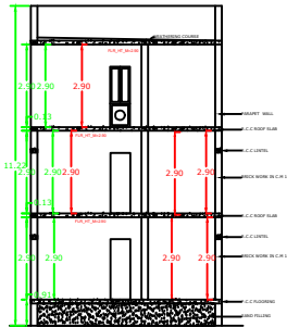
SECTION ON K-S
