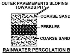
RAINWATER PERCOLATION BED
