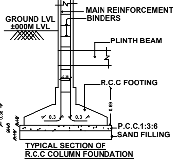
TYPICAL SECTION OF R.C.C COLUMN FOUNDATION
