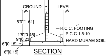
FOUNDATION DETAILS
