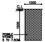
SECTION I PEBBLE TR SCALE : 1: =
