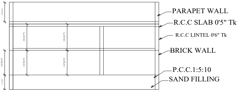
SECTION ON"AB"
