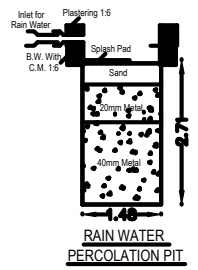
RAIN WATER PERCOLATION PIT
