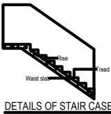
DETAILS OF STAIR CASE
