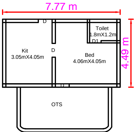
FIRST FLOOR (Prop)
