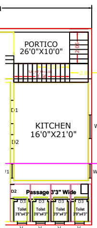
FLOOR PLAN
