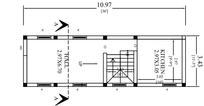
EXT.GROUND FLOOR
