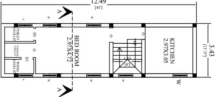
EXT.FIRST FLOOR
