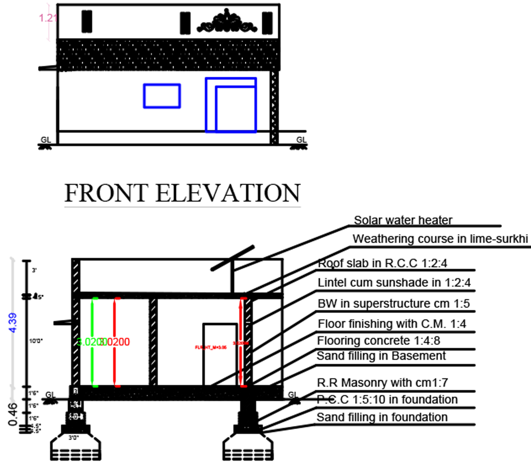
SECTION
