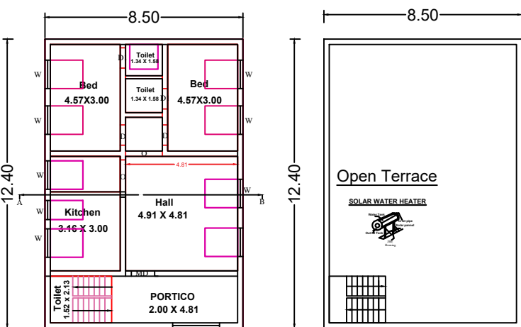
GF PLAN OPEN TERRACE
