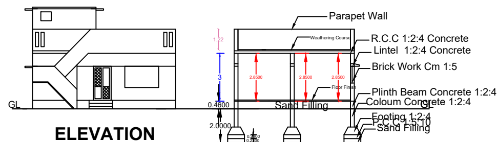
ELEVATION CUT SECTION ON AB
