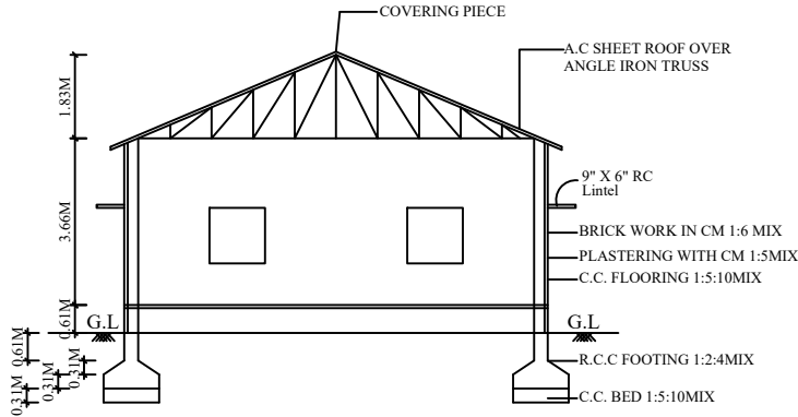
SECTION ON 'SP'
