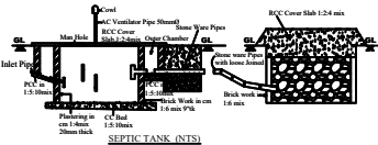
SEPTIC TANK (NTS)
