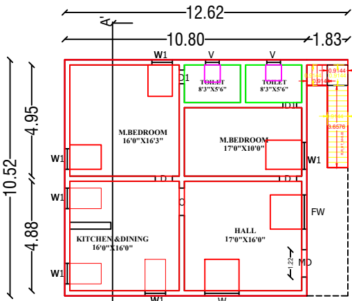
GROUND FLOOR PLAN FACING NORTH
