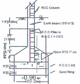
FOUNDATION DETAILS
