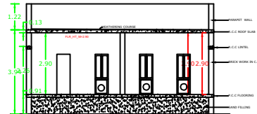
SECTION ON K-S
