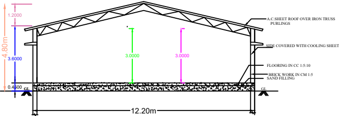
FRONT ELEVATION
