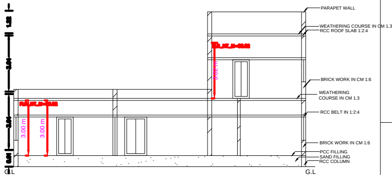
SECTION ON-AA&BB
